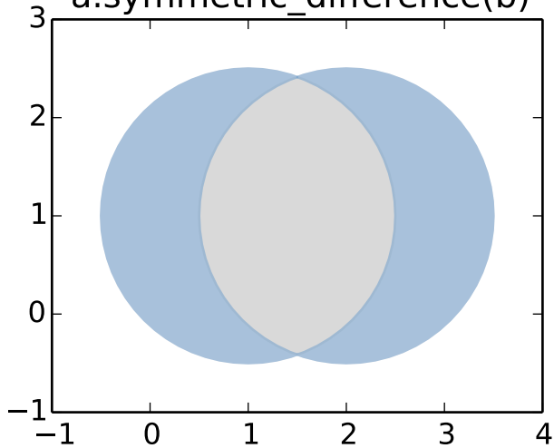
a.symmetric_difference(b)
