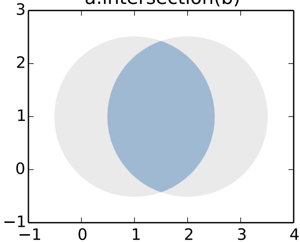
a.intersection(b)
