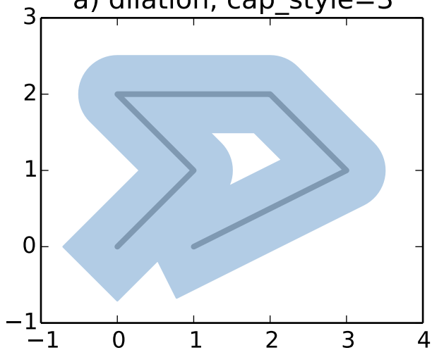
a) dilation, cap_style=3
